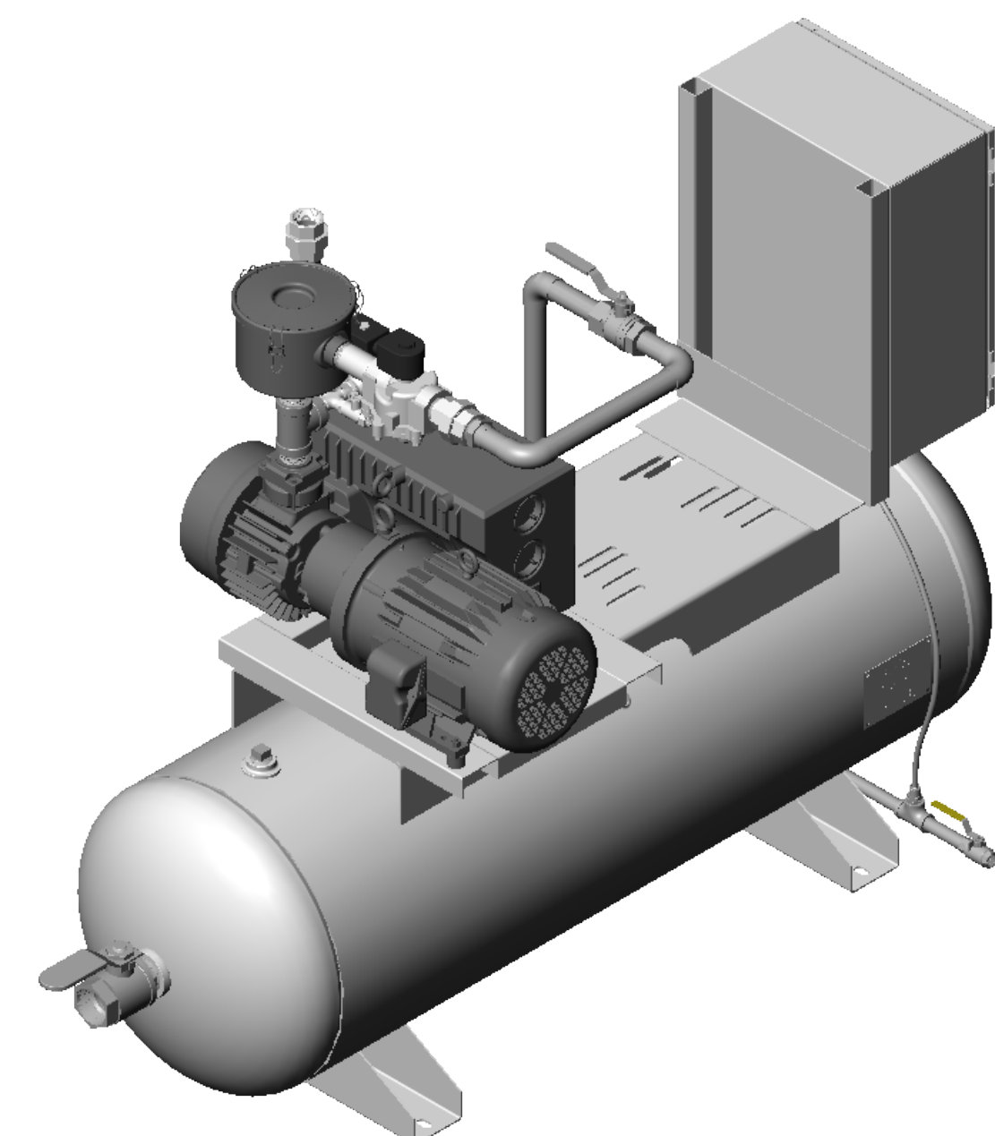
Isometric View (Back)
