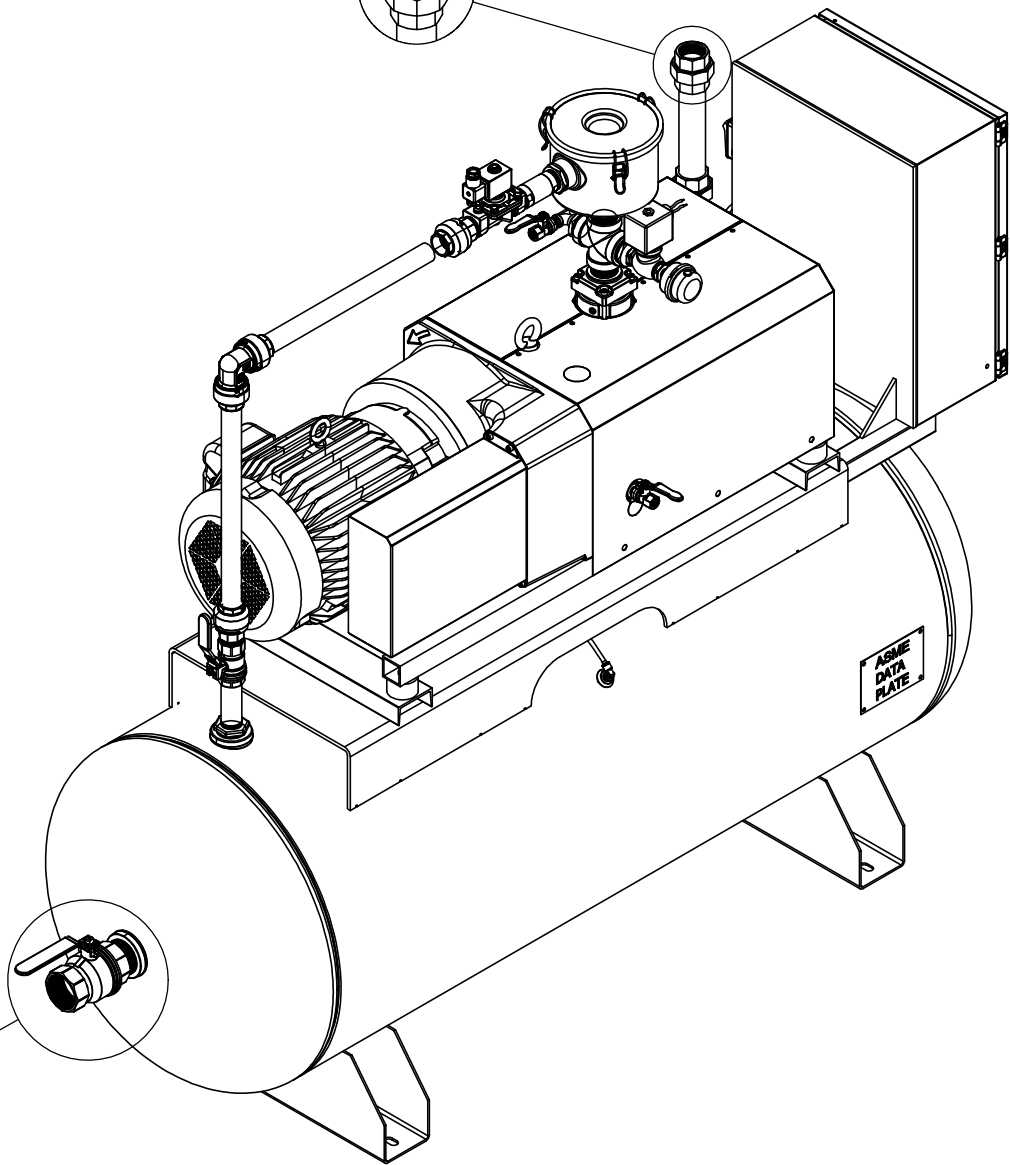
BACK ISOMETRIC VIEW
