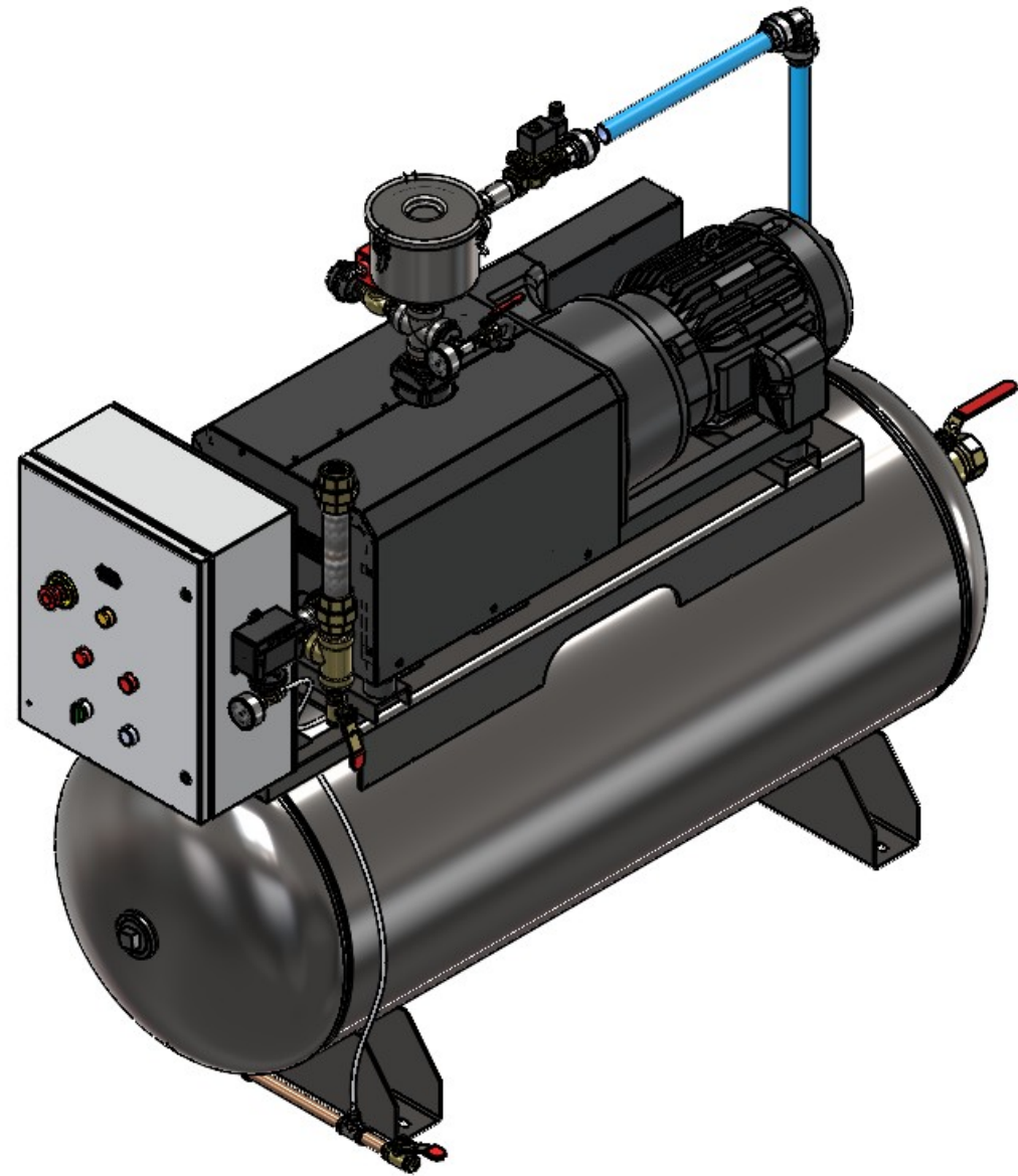
FRONT ISOMETRIC VIEW
