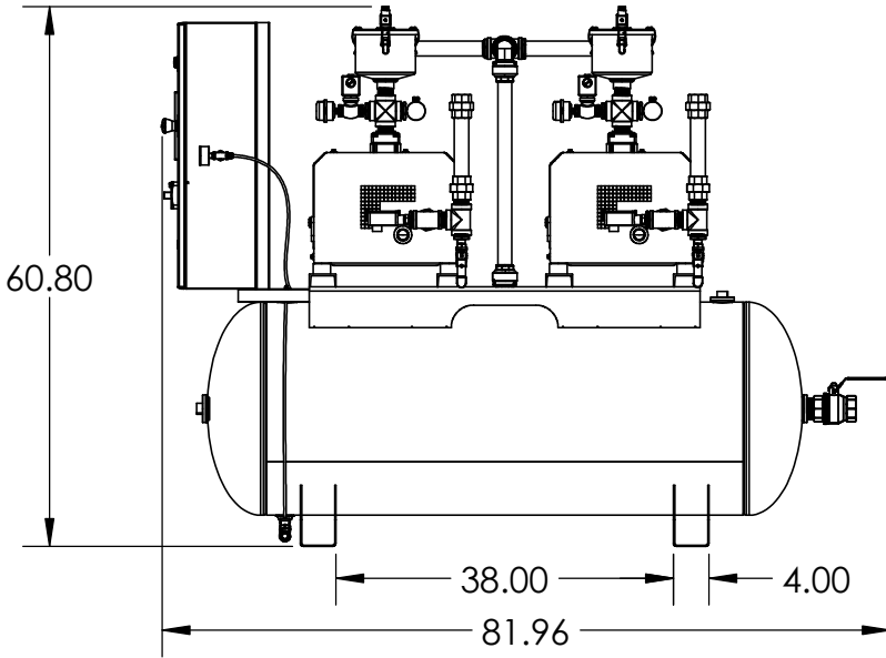
RIGHT VIEW
