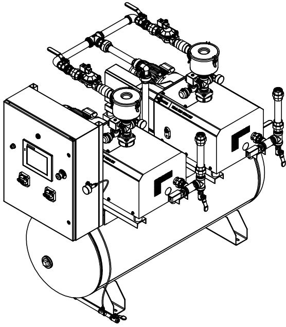
FRONT ISOMETRIC VIEW
