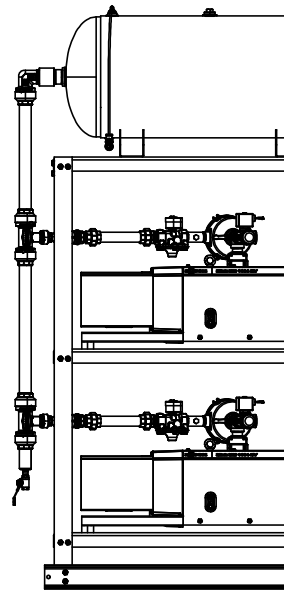
LEFT VIEW
