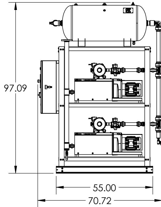
RIGHT VIEW
