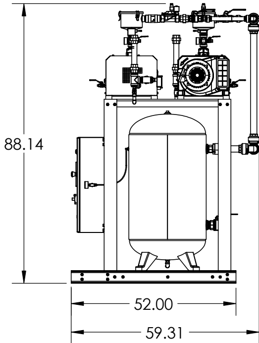
RIGHT VIEW
