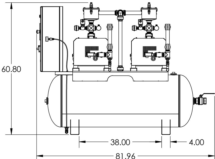
RIGHT VIEW
