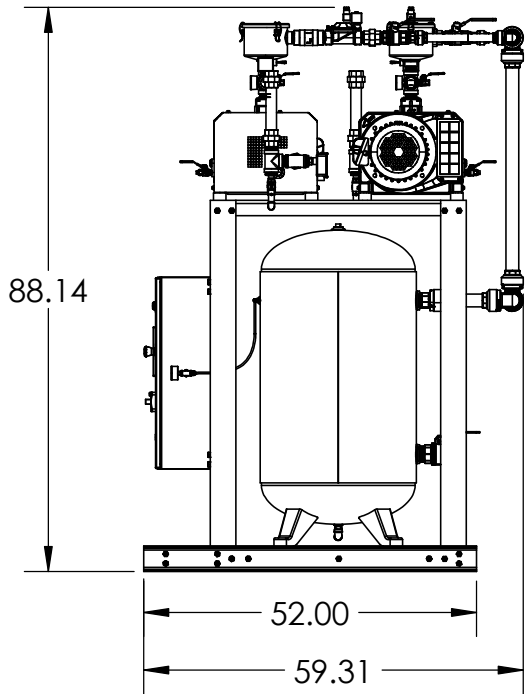
RIGHT VIEW
