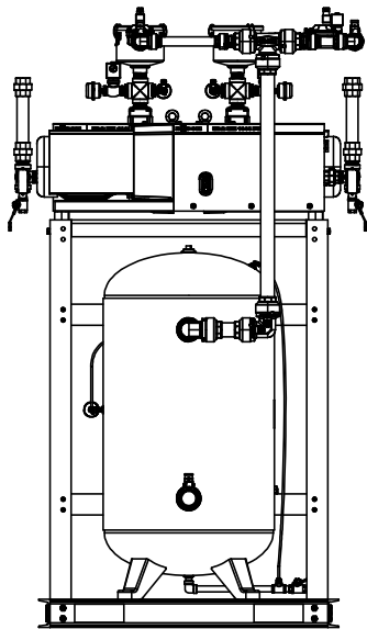
BACK VIEW
