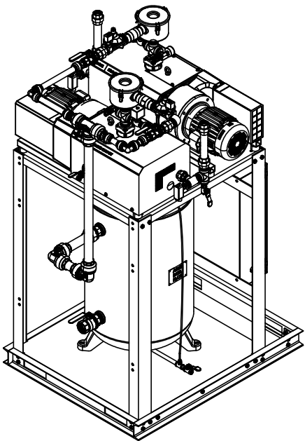
BACK ISOMETRIC VIEW
