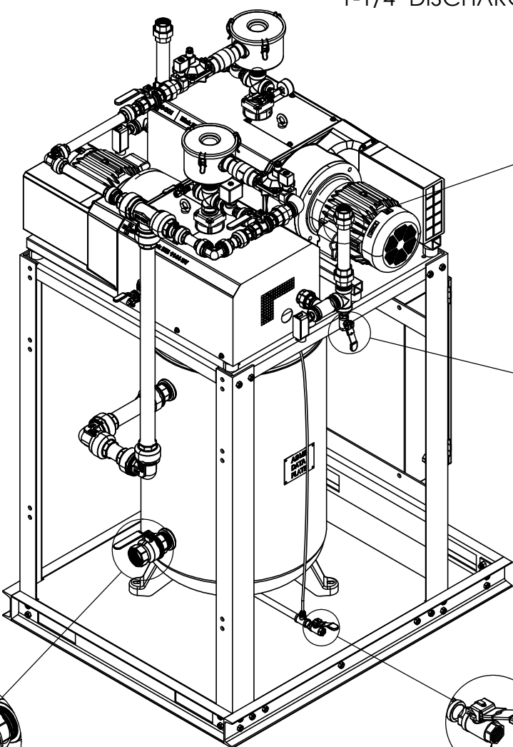
BACK ISOMETRIC VIEW
