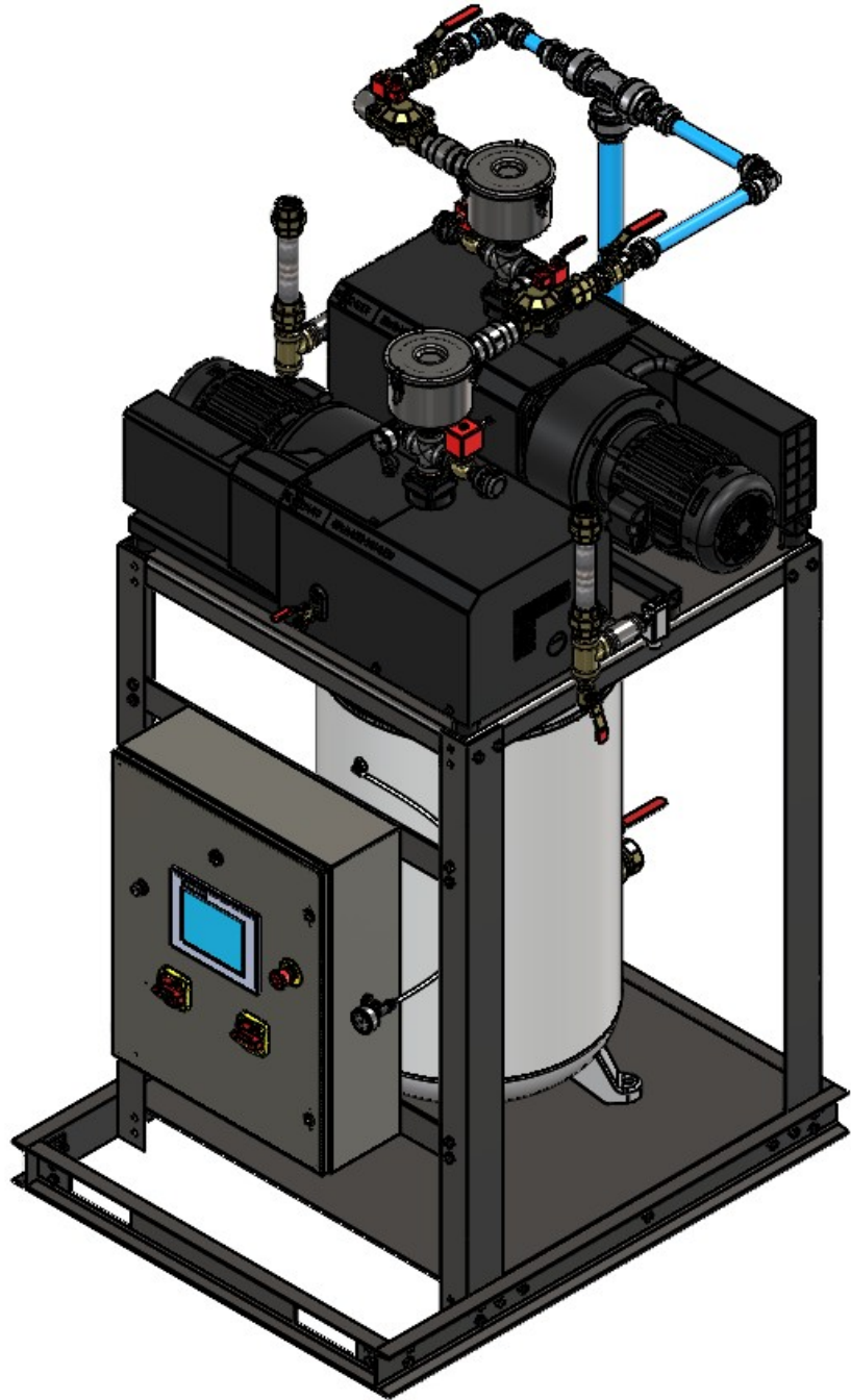
FRONT ISOMETRIC VIEW
