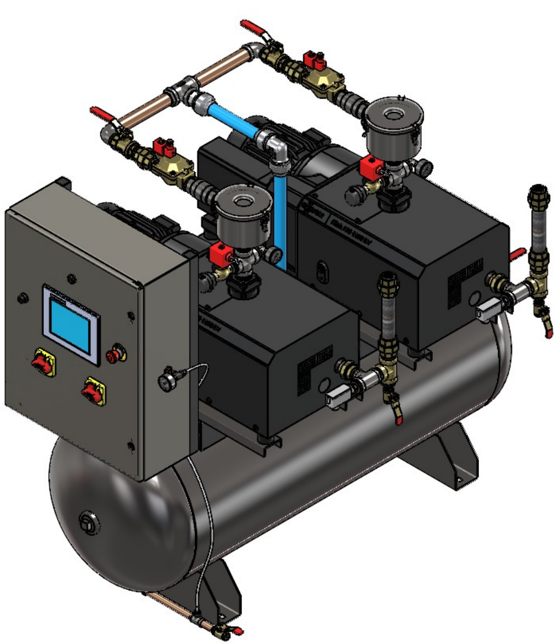
FRONT ISOMETRIC VIEW
