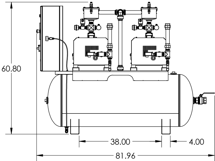
RIGHT VIEW
