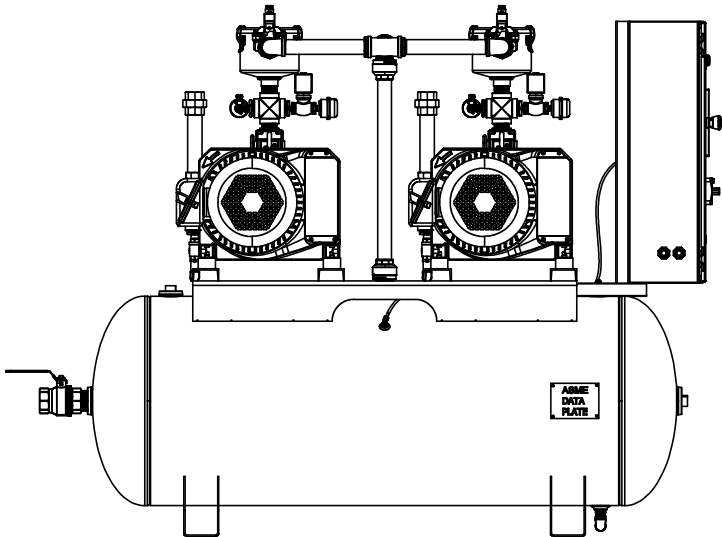
LEFT VIEW
