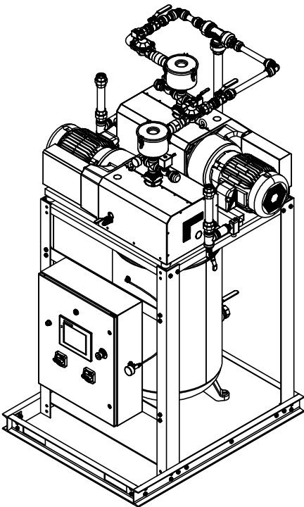
FRONT ISOMETRIC VIEW
