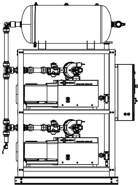
LEFT VIEW
