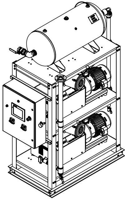
FRONT ISOMETRIC VIEW
