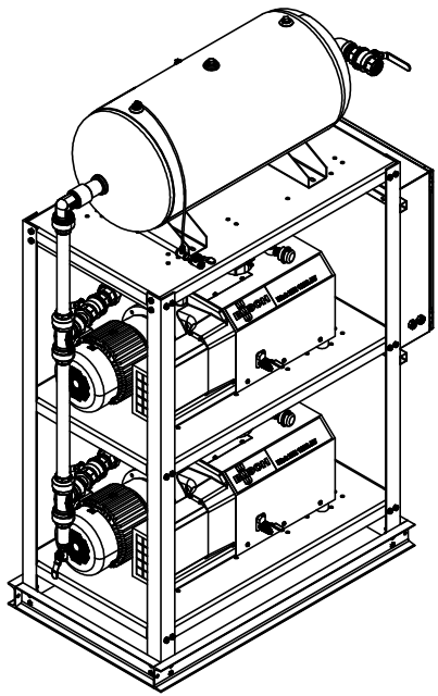
BACK ISOMETRIC VIEW
