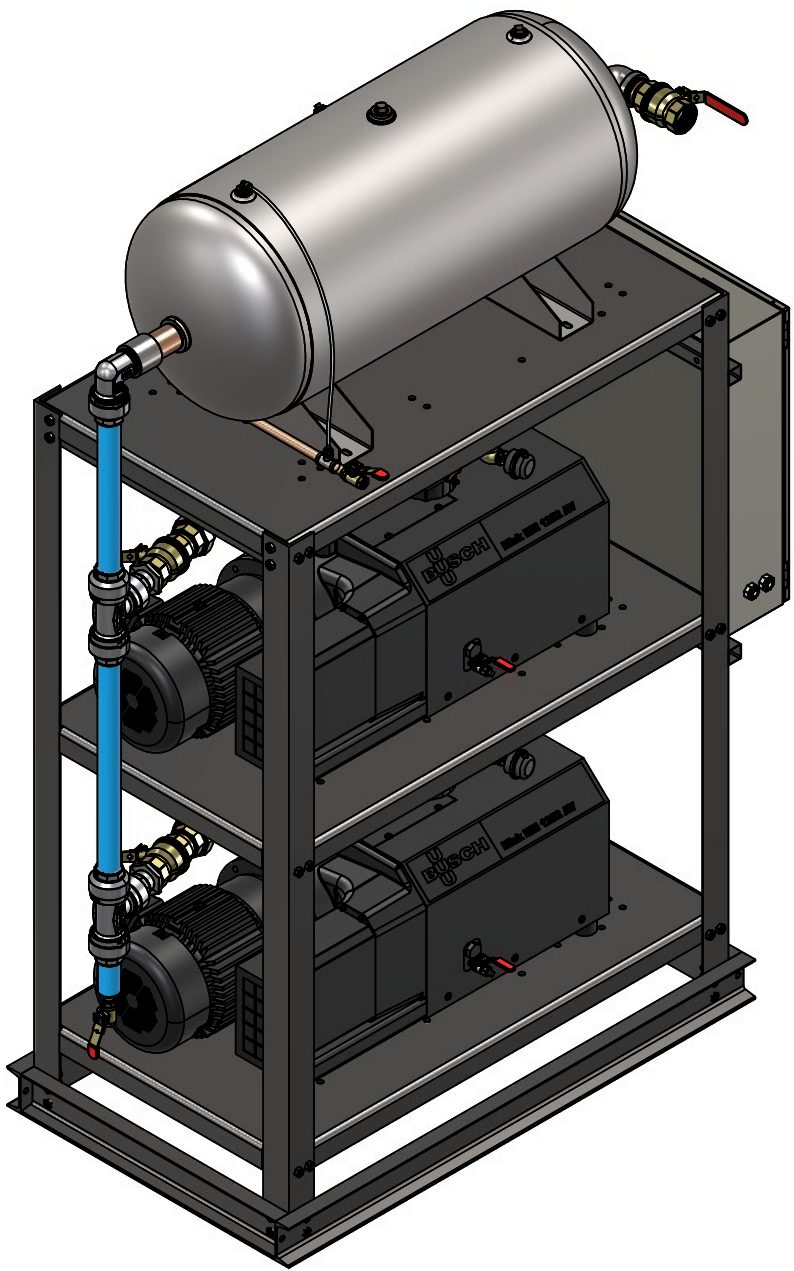
BACK ISOMETRIC VIEW
