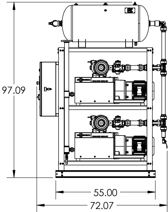
RIGHT VIEW
